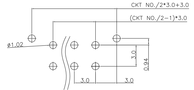
RECOMMENDED PCB LAYOUT COMPONENT SIDE(TOL: ±0.05mm)
